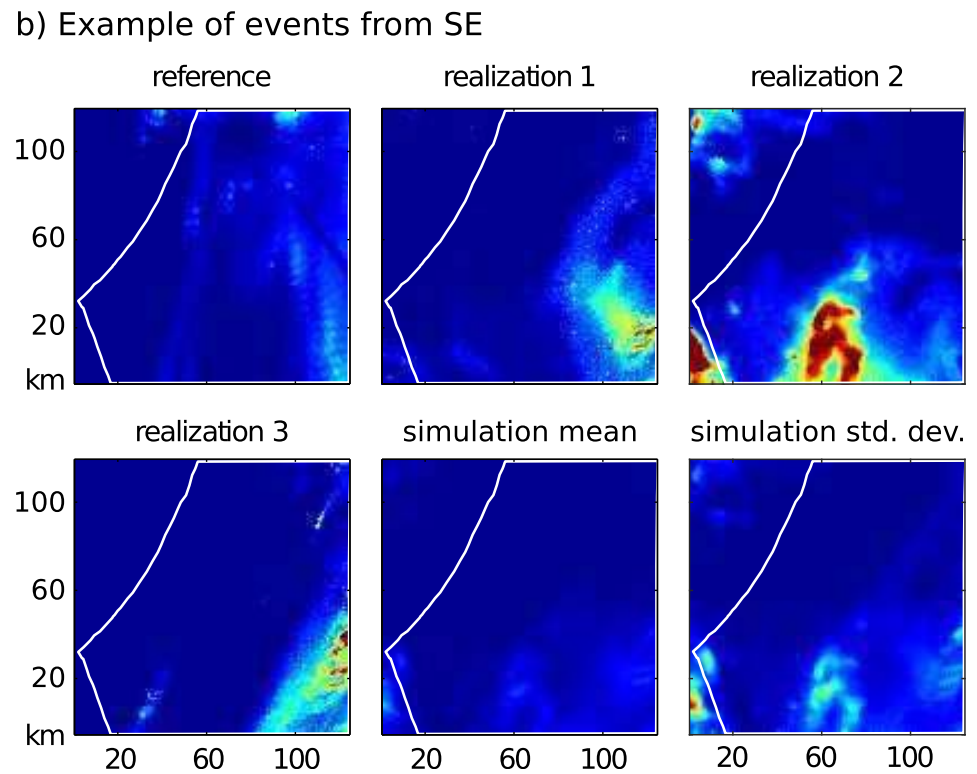
Figure 7. Visual comparison of the daily rainfall fields for the (a) NW and (b) SE classes. For both Figures 7a and 7b, one daily reference field is shown together with three simulated fields, the mean and standard deviation of the simulation ensemble for the reference day. The white line represents the shore line and study region perimeter.
