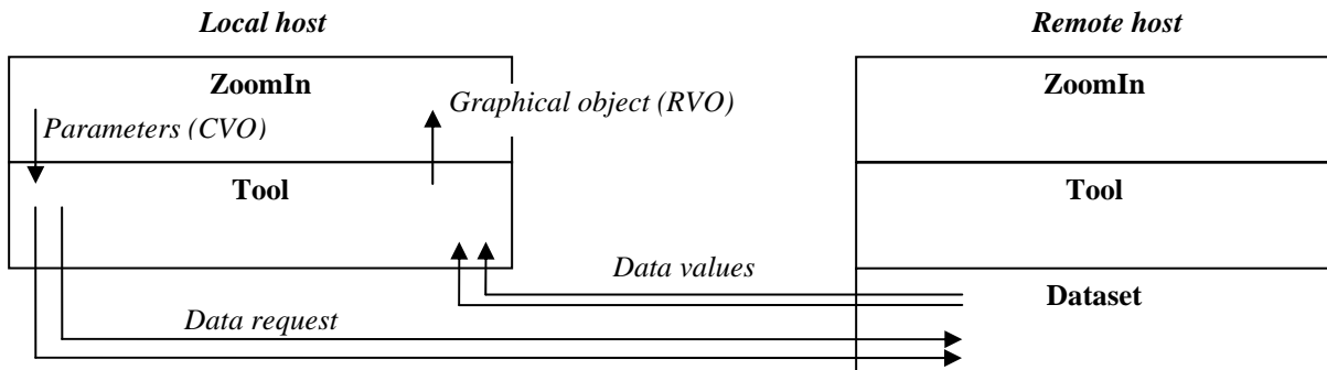
Figure 5. "Remote dataserver": Dataset not available on the local host and computation of the dataset on a remote host
