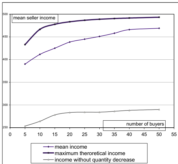
Figure 4: Vendor revenue in relation to the number of buyers.
