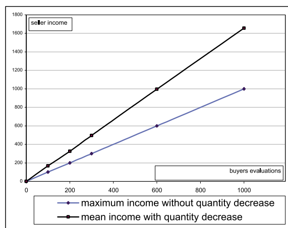
Figure 3: Vendor revenue in case of heavy competition.
