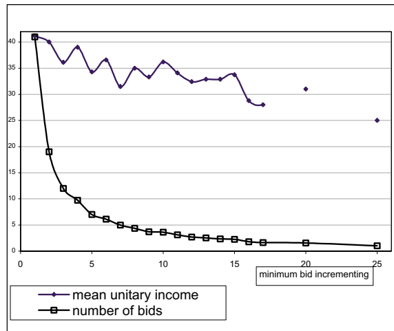
Figure 5: Vendor revenue and number of bids in relation to the minimal bid increment value.
