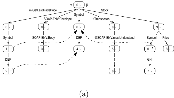
Figure 3: XTrie for the sample XPath expressions of Section 2.2. (a) Trie. (b) Auxiliary table.
