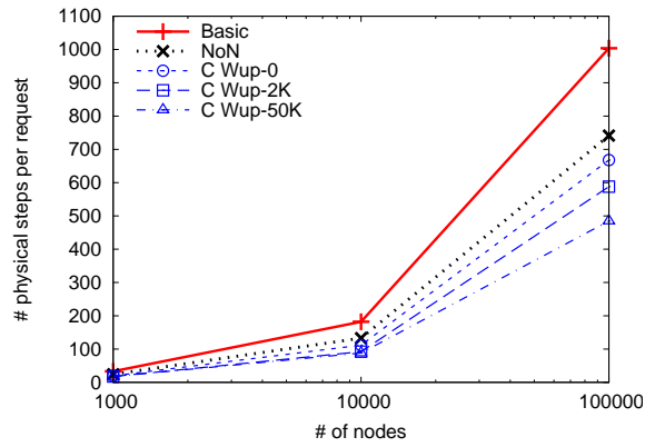
Fig. 2. Average number of physical steps to achieve a request
