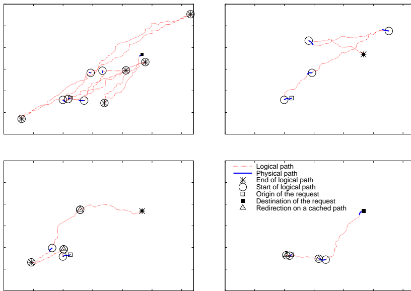
Fig. 5. Path of a request with Basic (top left), NoN (top right), C Wup-2K (bottom left), and C Wup-50K (bottom right) in a two-dimensional space.
