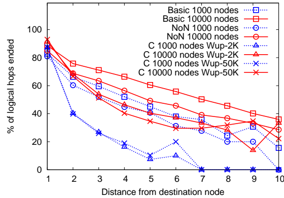
Fig. 4. Percentage of terminated logical hops
