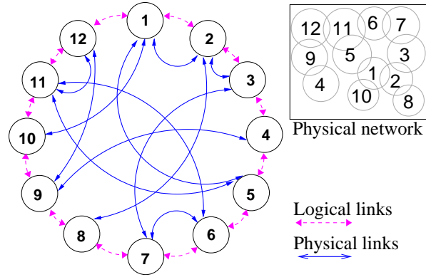
Fig. 1. Illustration of the DHT model for ad-hoc network.
