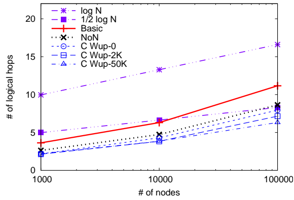
Fig. 3. Average number of logical hops per lookup
