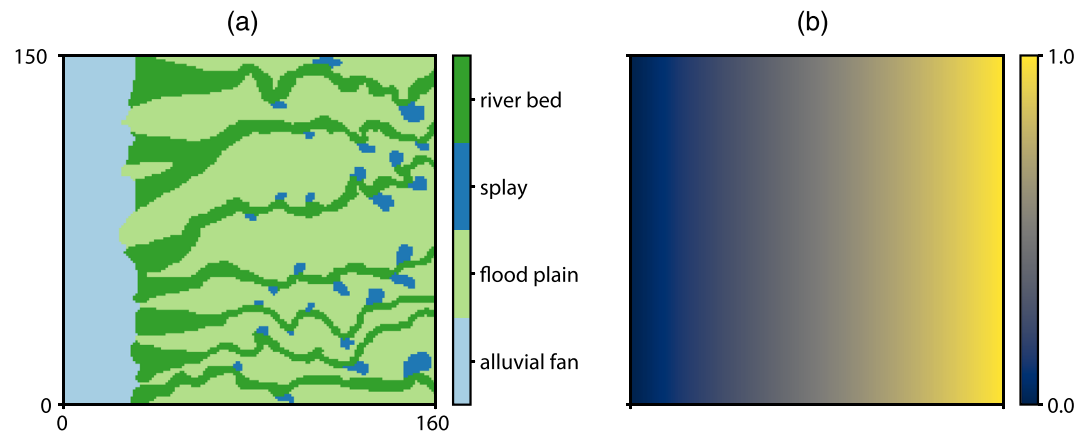
Figure 10. The analog training image (a) with its corresponding trend (b). The training image contains four geological facies.
