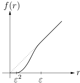
FIGURE 1. The “cut off” function f .
