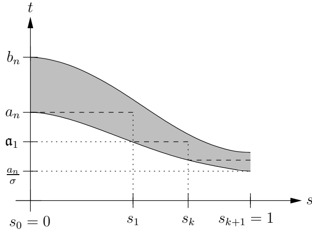
FIGURE 3. The curves a_n(s) and b_n(s) .
