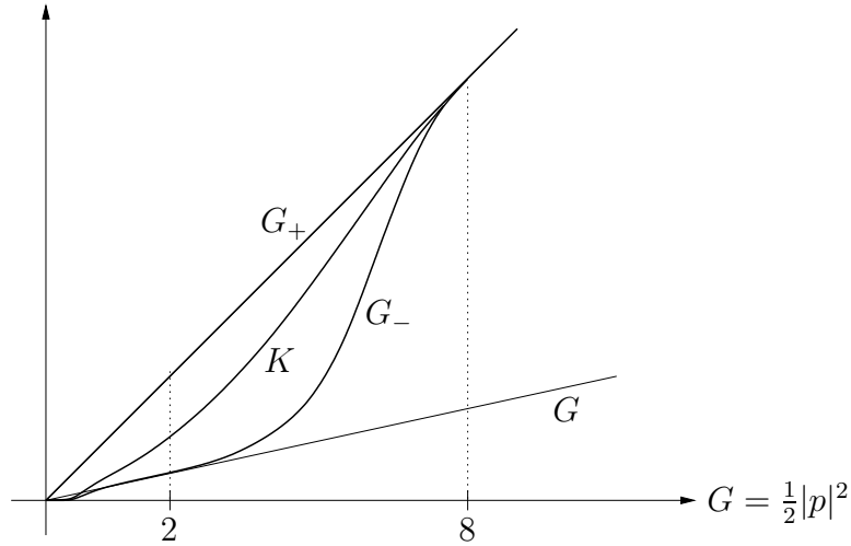
FIGURE 2. The functions G_- \leq K \leq G_+ , schematically.
