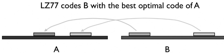
Figure 2. Scheme of the LZ77 algorithm when comparing two different texts. Instead of concatenating the two texts and zipping them sequentially (which would imply that the compressor first learns A, then for a “while” (see (Benedetto et al., 2002) ) measures the cross-entropy between B and A and then learns B), one always scans B. In the refined scheme the compressor does not zip the B part but simply ‘reads’ it with the (almost) optimal coding of part A. In this case we start reading sequentially file B and search in the look-ahead buffer of B for the longest subsequence that already occurred only in the A part. This means that we do not allow for searching matches inside B itself. As in the usual LZ77, every matching found is replaced with a pointer indicating where, in A, the matching subsequence appears and its length.
